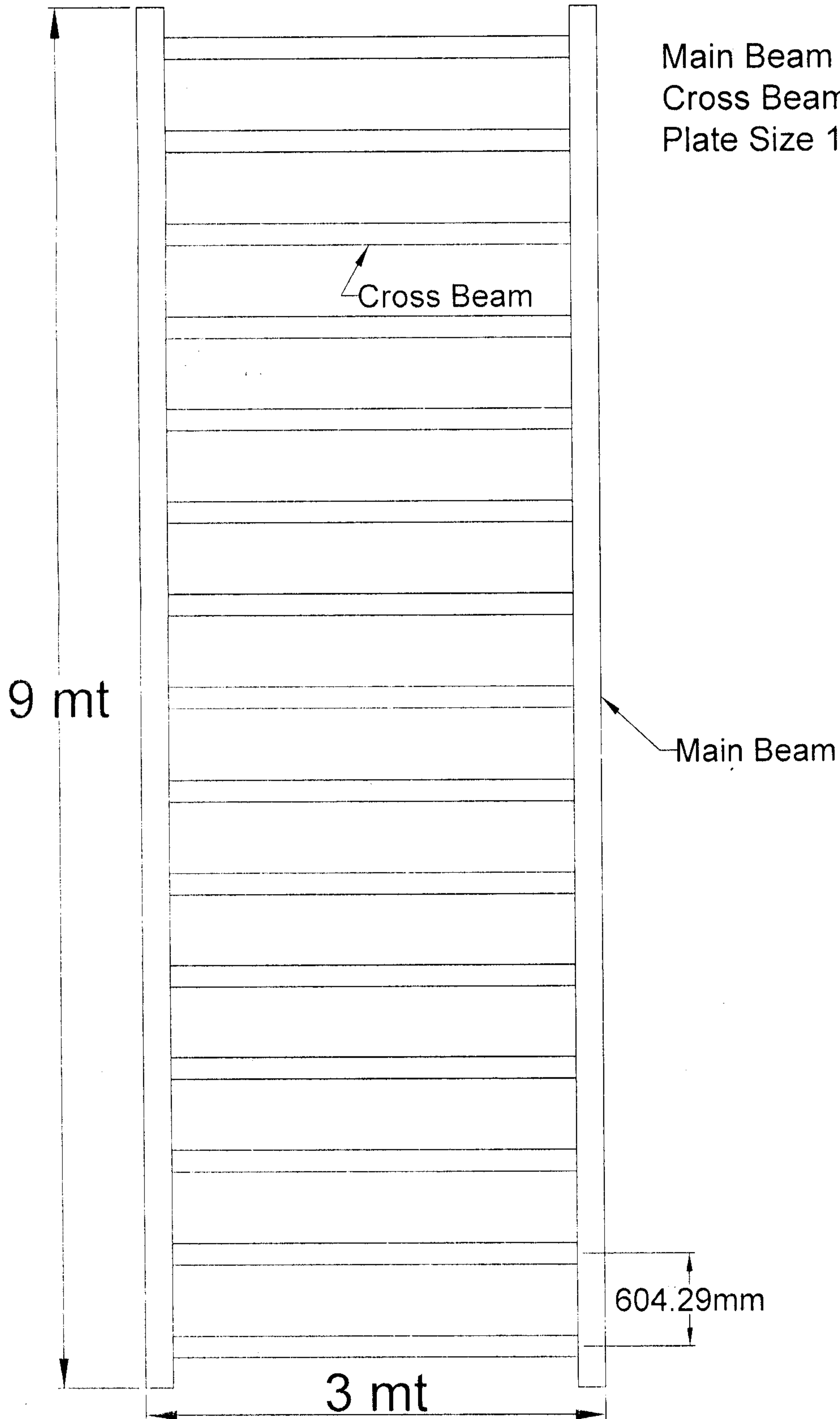
Weighbridge Structure
